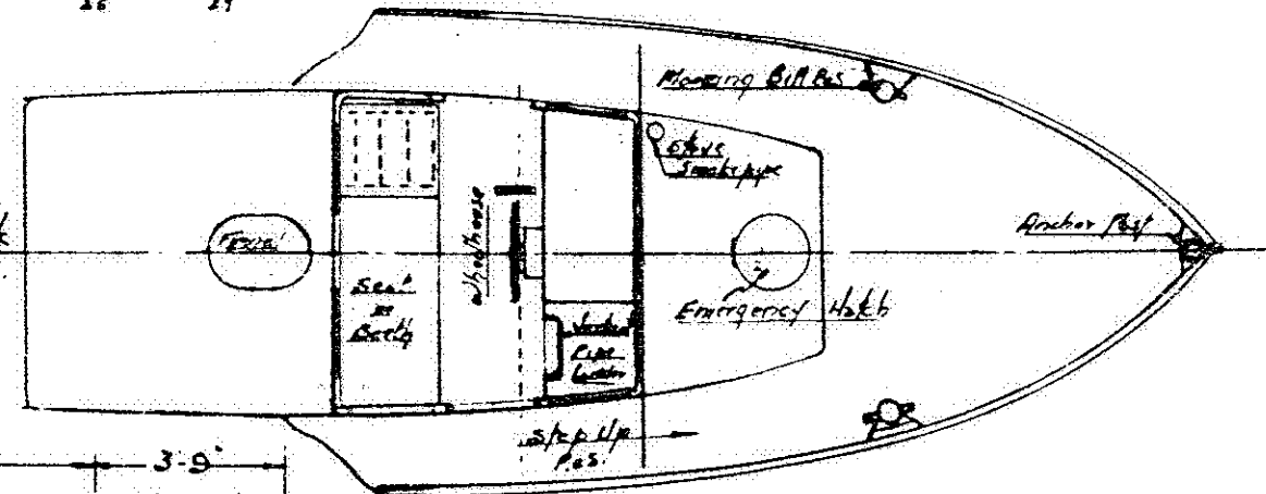
WHEELHOUSE & FORE DECK
