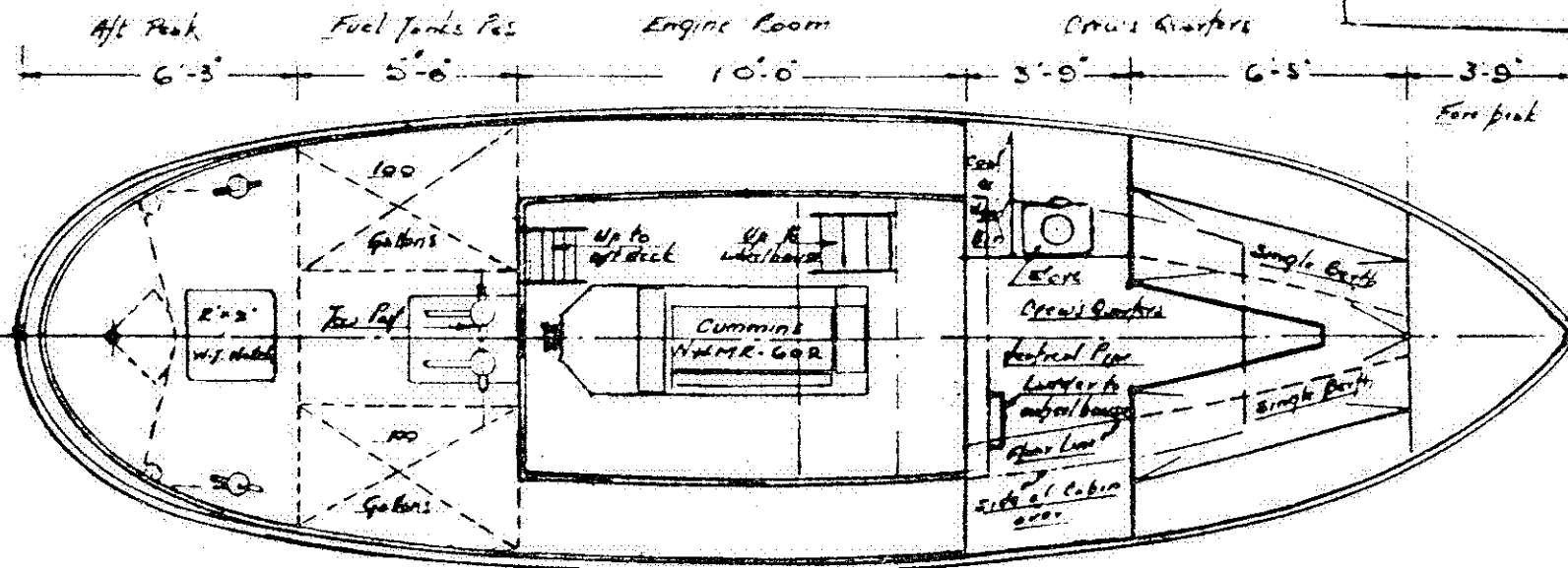
MAIN DECK, ENGINE ROOM & ACCOMMODATION
